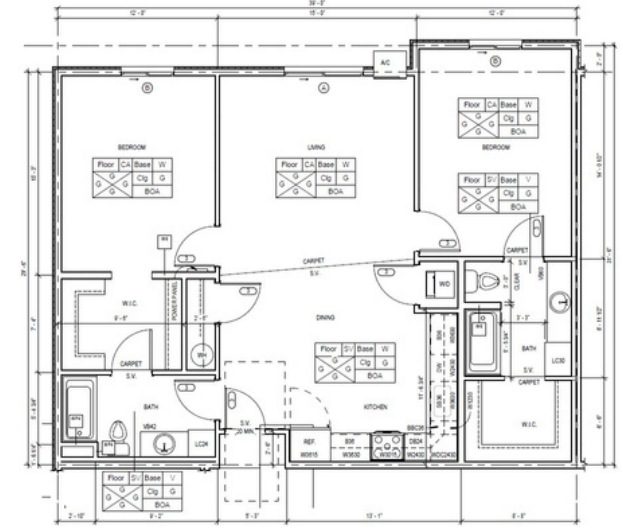
Unit 2B3-B Type: B 1,115 SF - 1.74US
