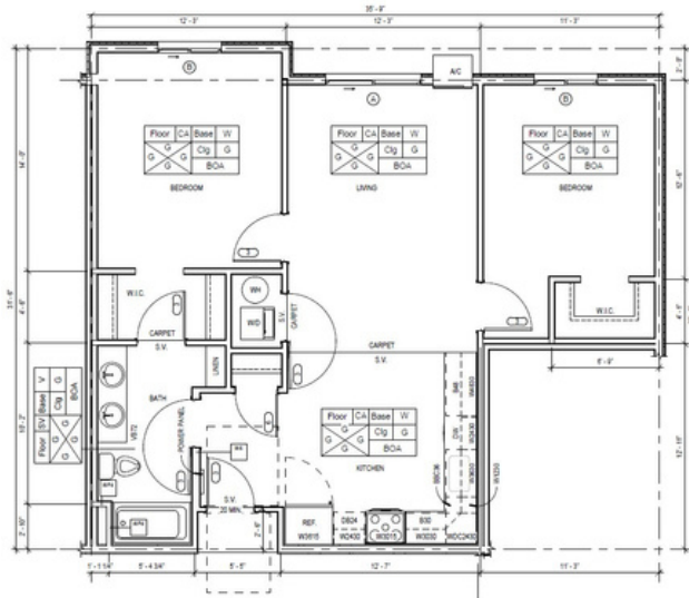
Unit 2B2-B Type: B 879 SF - 1.74US
