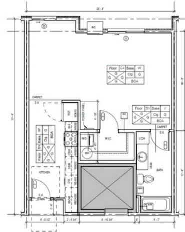
Unit Studio-B Type: B 585 SF - 2.74US
