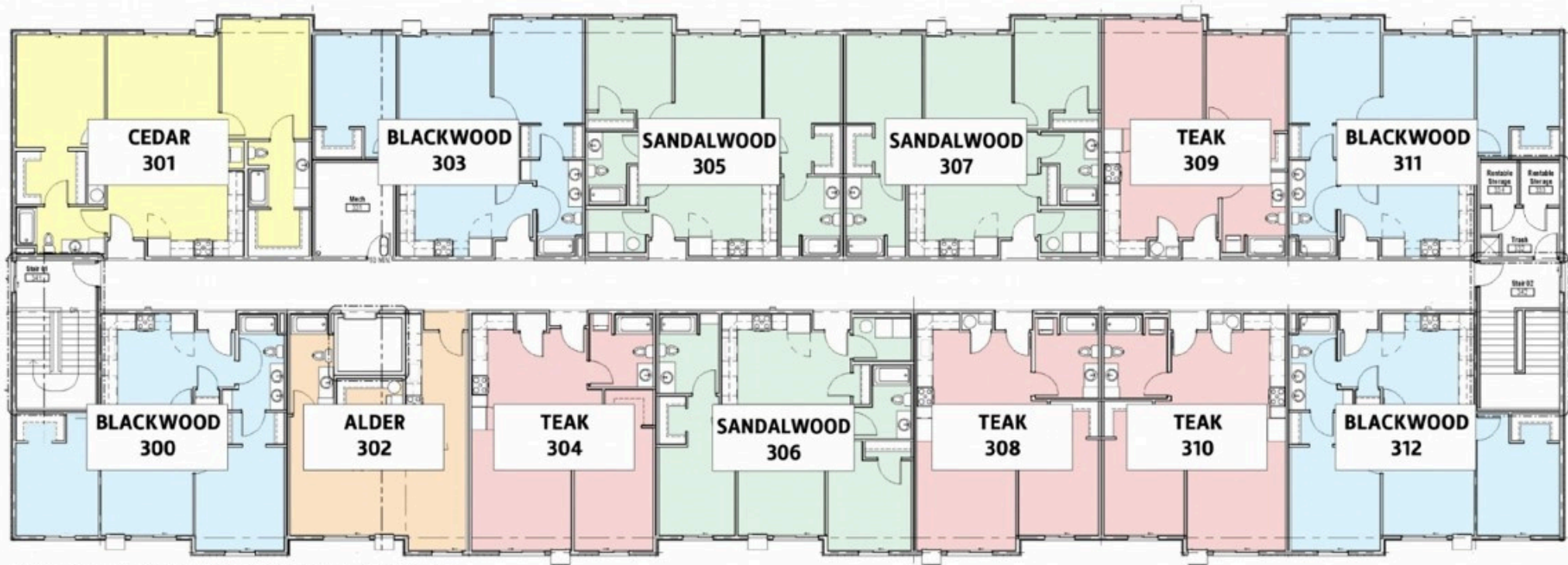
THIRD FLOOR APARTMENT PLAN
