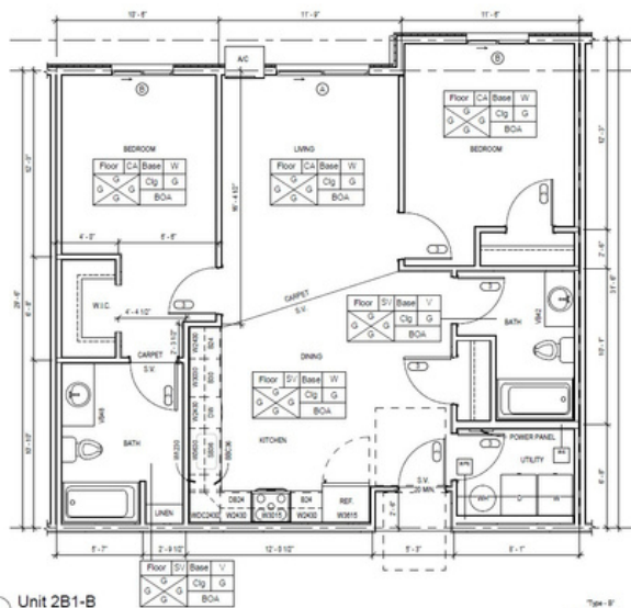
Unit 2B1-B Type: B 948 SF - 0.74US
