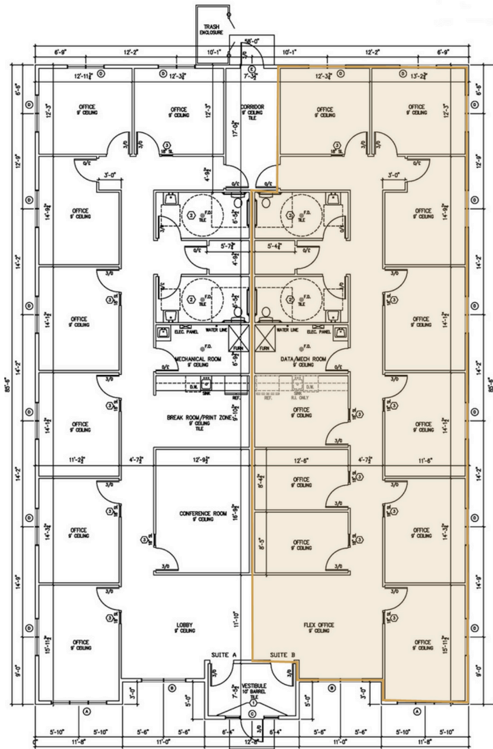
FLOOR PLAN 1/8"=1'-0" 4918 SF
